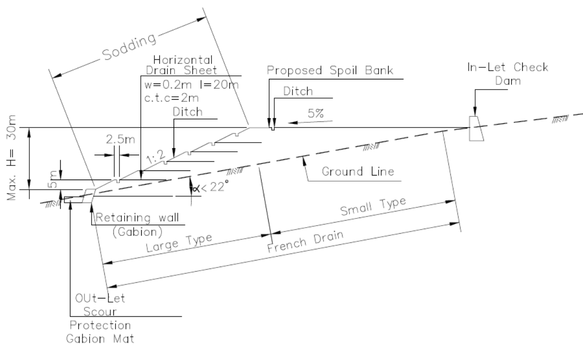
Figure-1(b): Typical Arrangement for Spoil Banks: Profile
